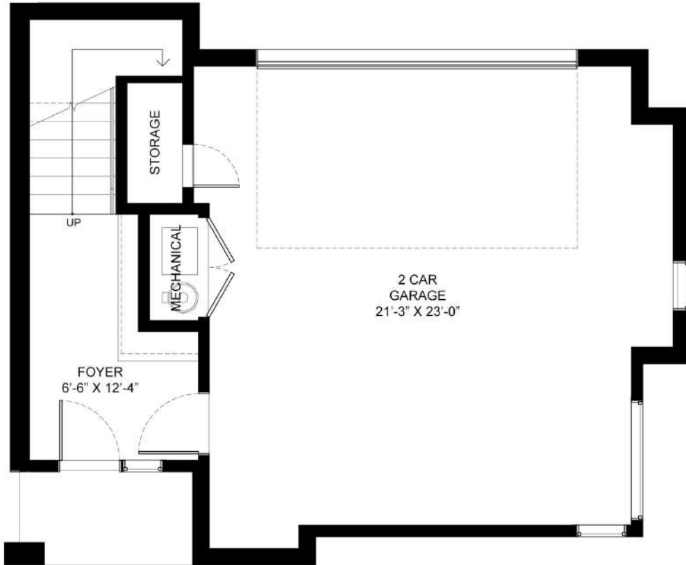
FIRST FLOOR PLAN - UNIT B
